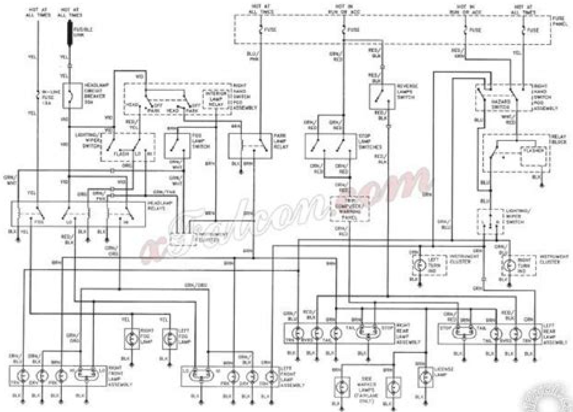
Typical 1979 through 1987 exterior lighting wiring diagram
