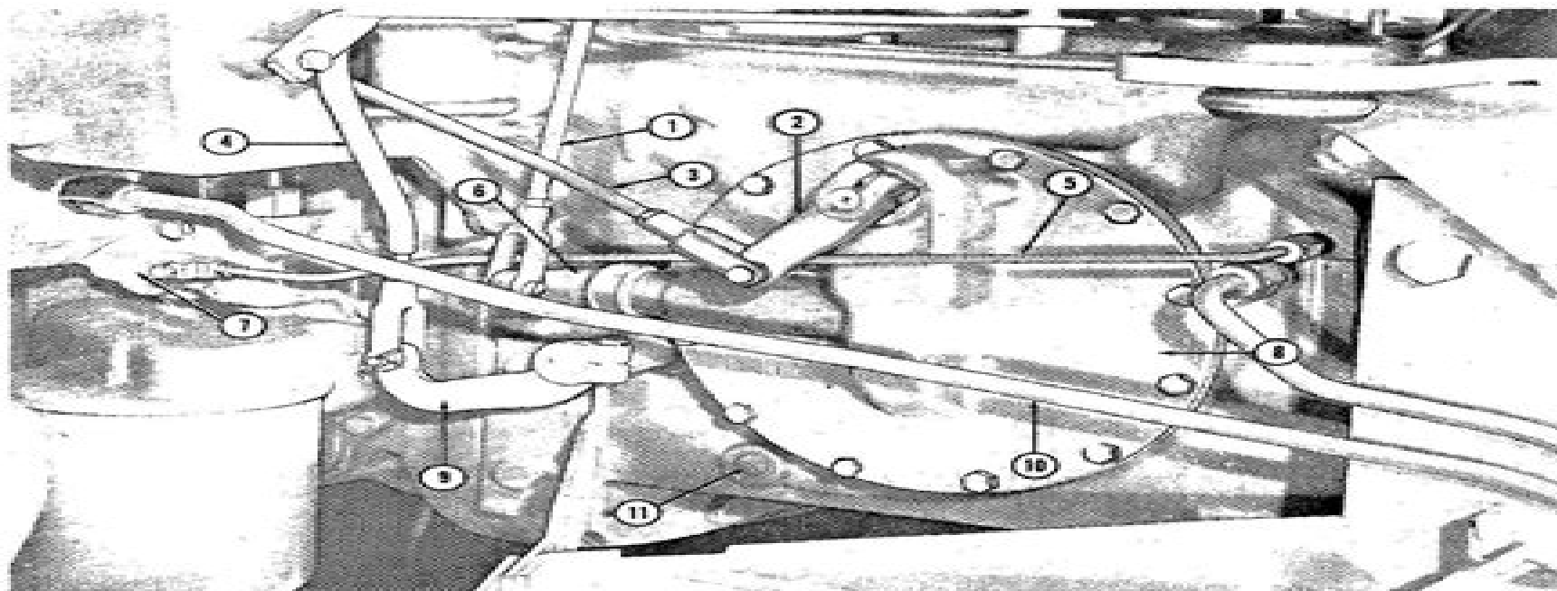
Figure 12 Right Side of Transmission
