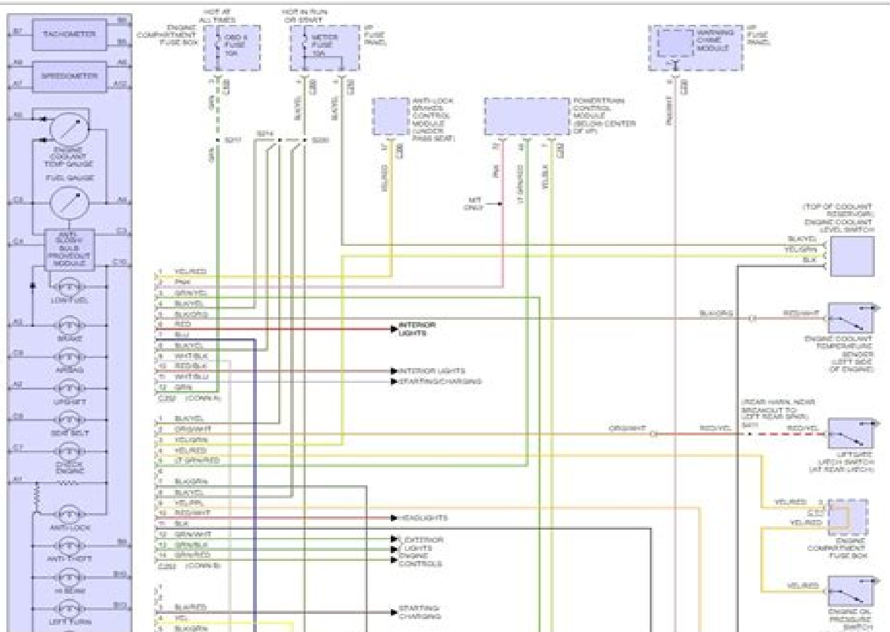
Fig 1: Instrument Cluster Circuit, Sport Cluster
