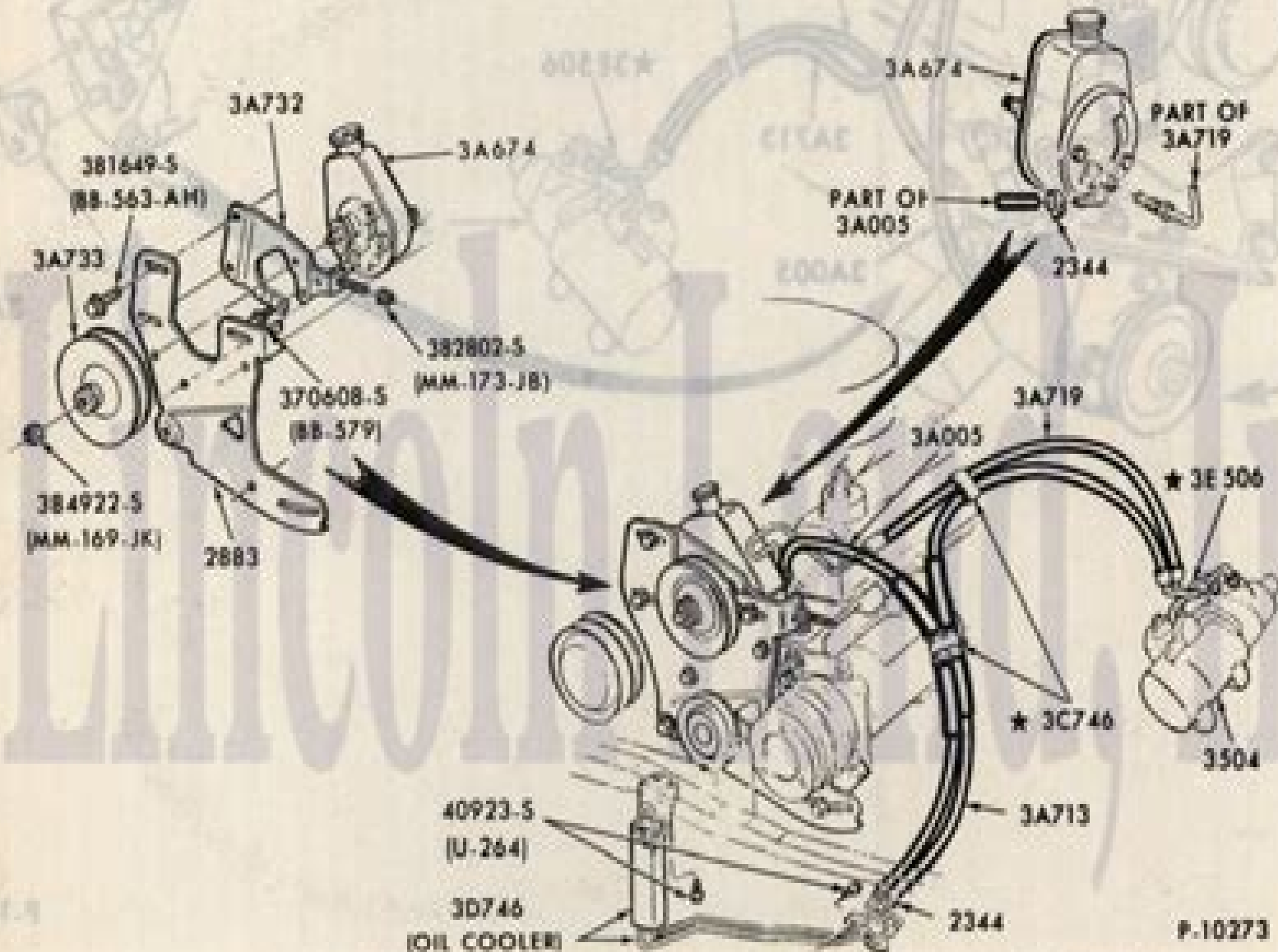
POWER STEERING HOSE and PUMP INSTALLATION-TYPICAL 1973/74 LINCOLN "BEFORE 4/8/74" and MARK IV (w/o HYDRO-BOOST)
