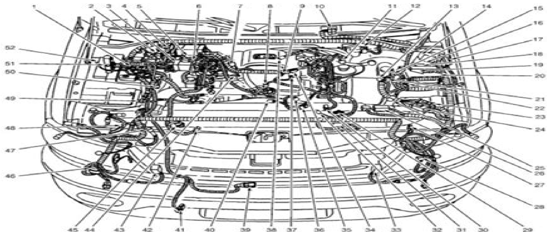
Fig 1: Engine Compartment
