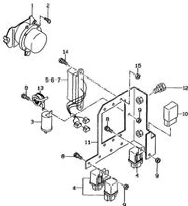
FIG. 16 ELECTRICAL PARTS(RELAY & HORN)
