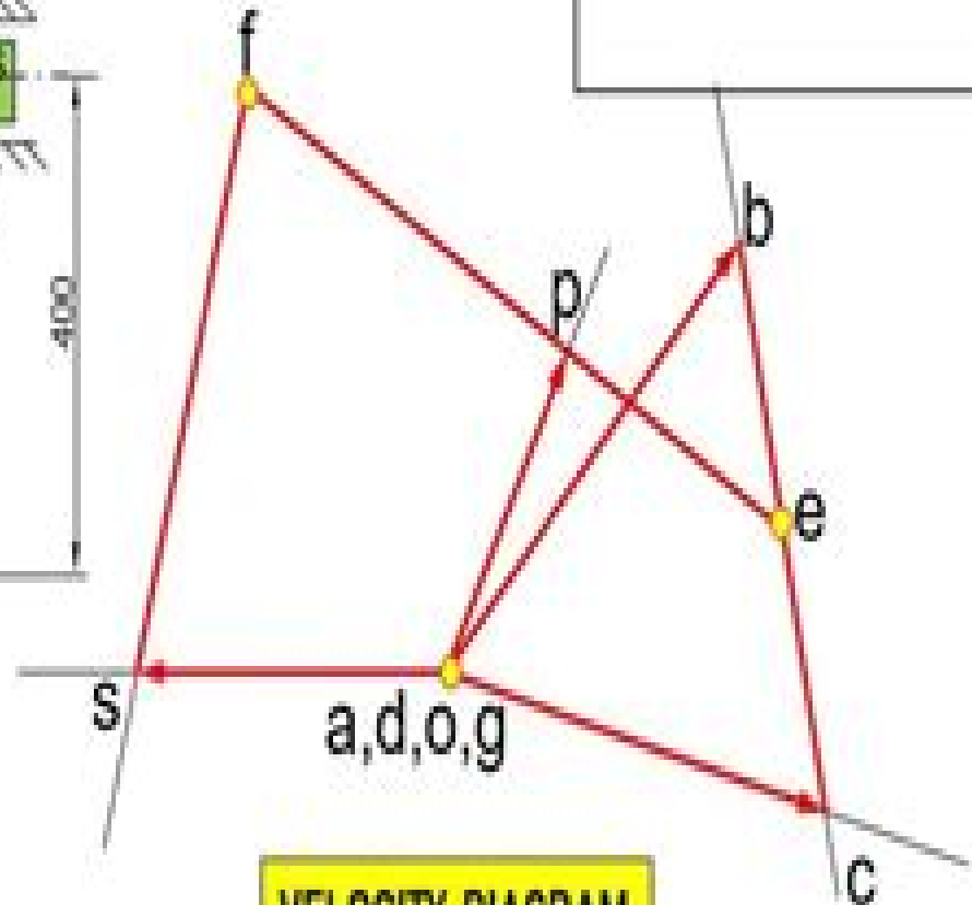
VELOCITY DIAGRAM
