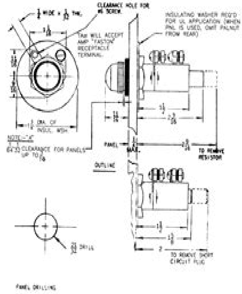
Figure 4 (continued): OUTLINE AND PANEL DRILLING FOR ROOM INDICATING LAMP TYPE ET-12
