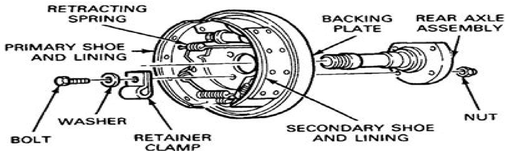
FIG. 10 Self Adjusting Brake Assemblies-Heavy Duty—E-250—E-350, F-250—F-350
