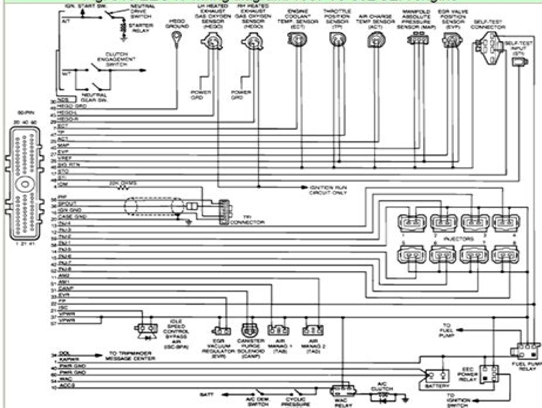
Fig. 318 EEC-IV wiring diagram, 1987 V8-302 SEFI engine
