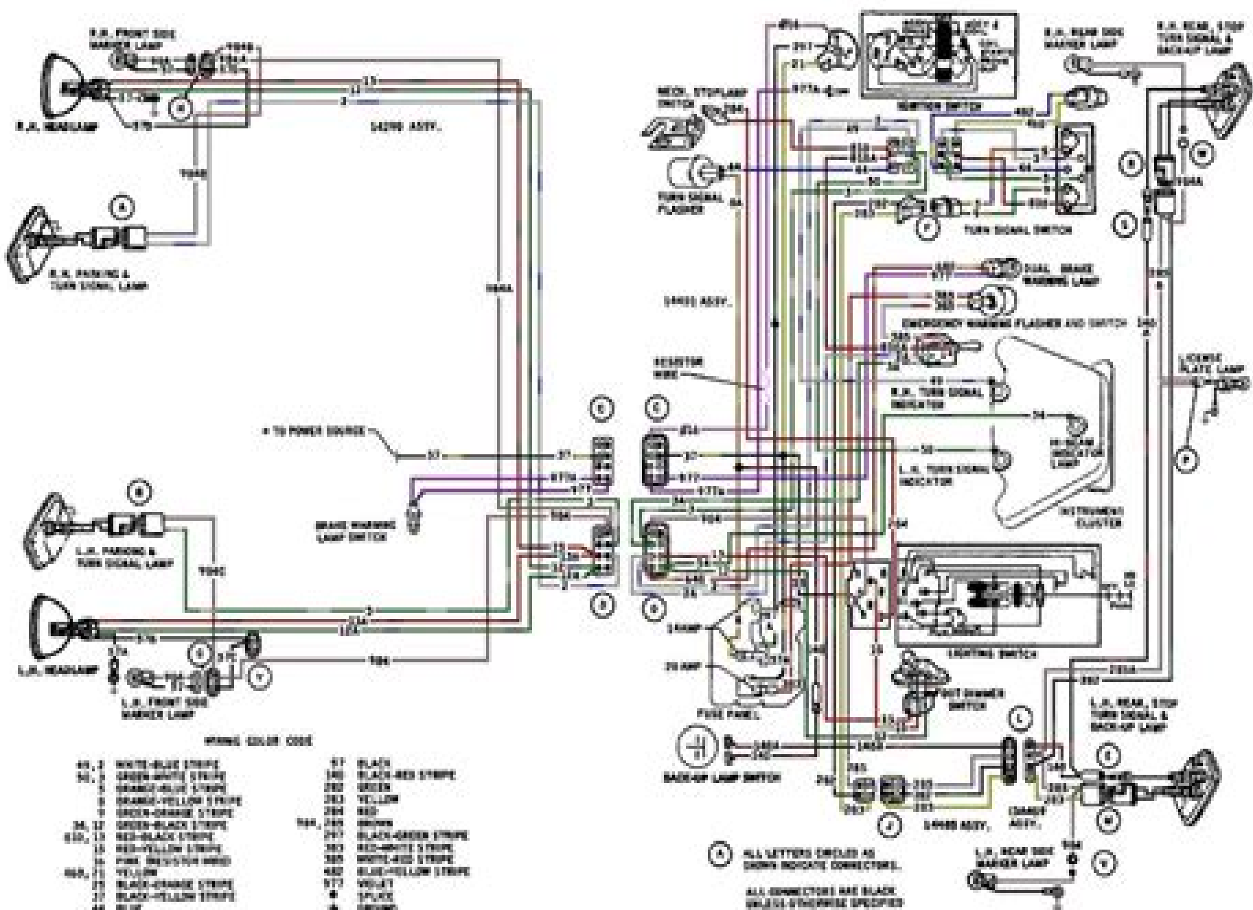
Wiring diagram for the exterior lights and turn signals—1970 Bronco *1970 is the latest
