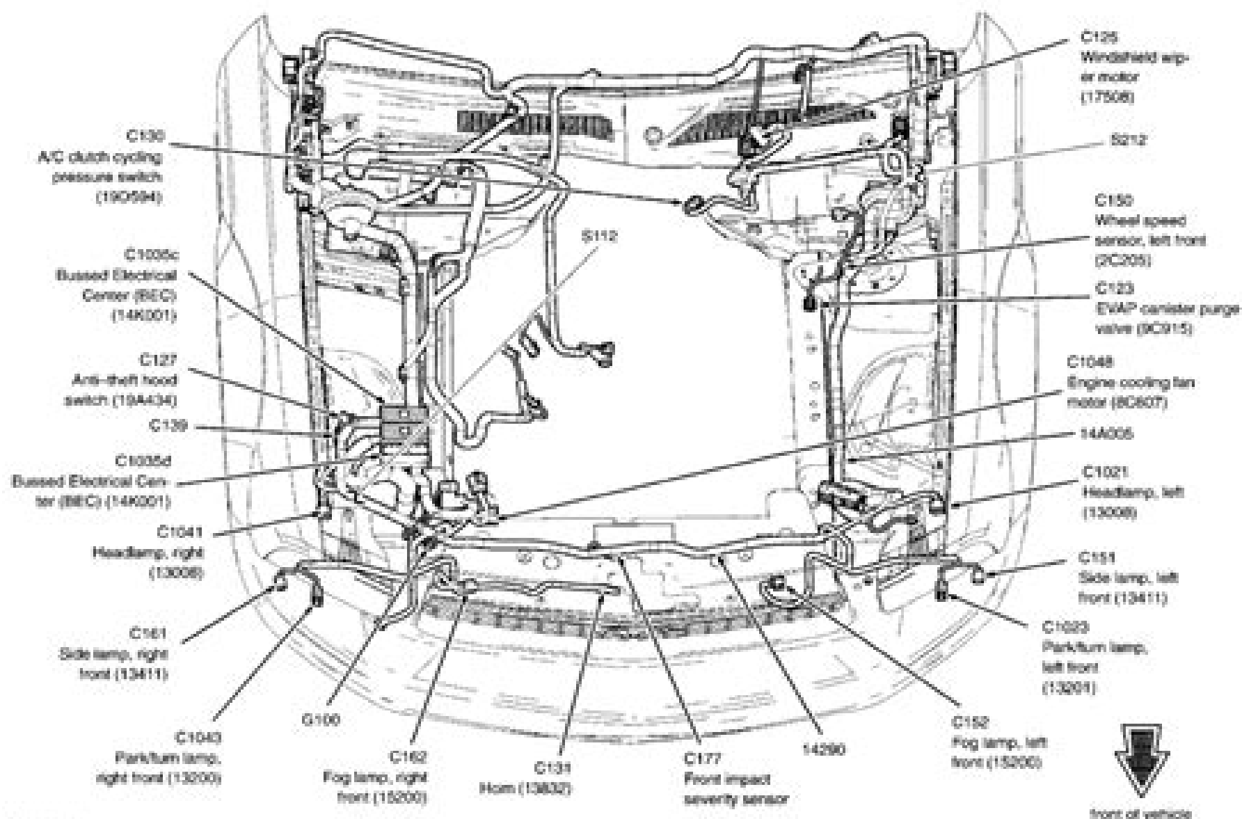
Fig 1: Engine Compartment
