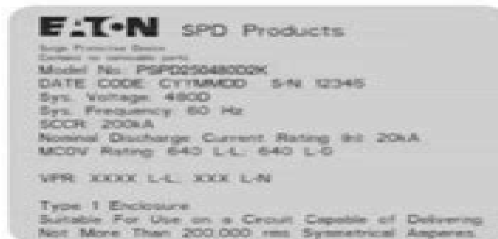
Figure 1. Product Label
