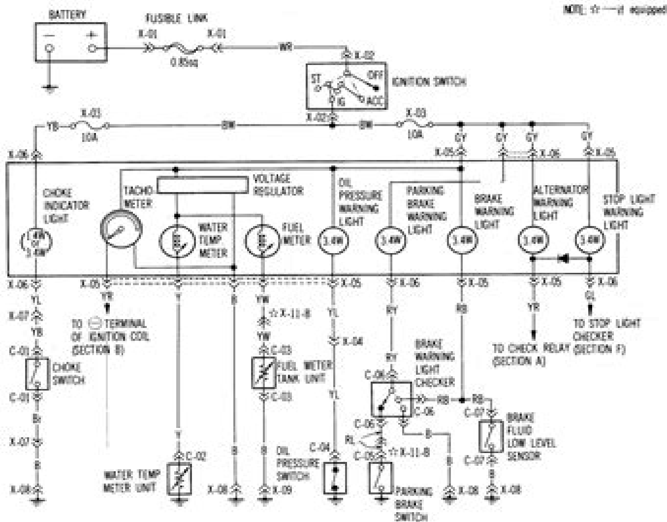
Instrument and warning light wiring diagram (1981 models)
