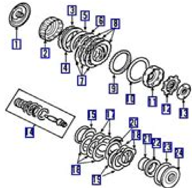
CLUTCHES & PLANETARY GEARS
