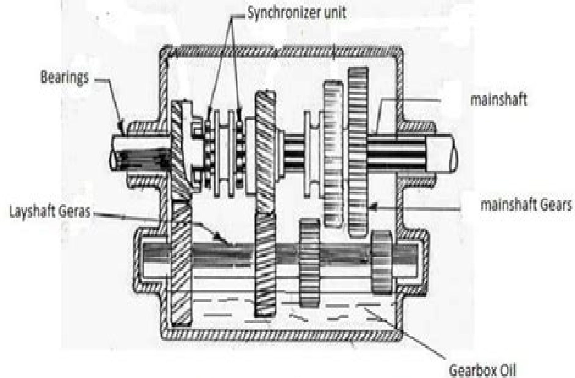
Fig:- Splash Lubrication of Synchromesh Gear box
