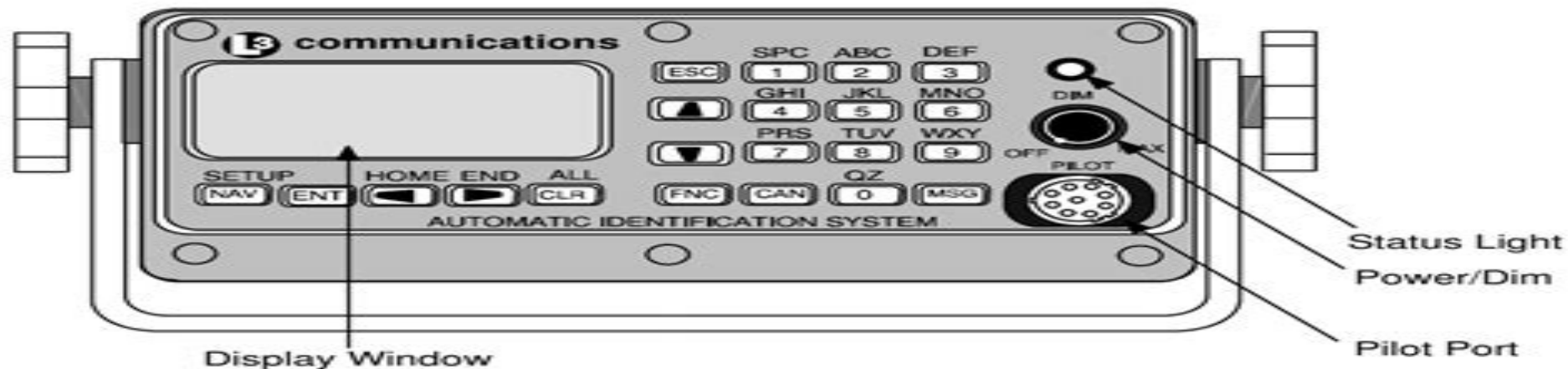
Figure 2-1. AIS Transponder
