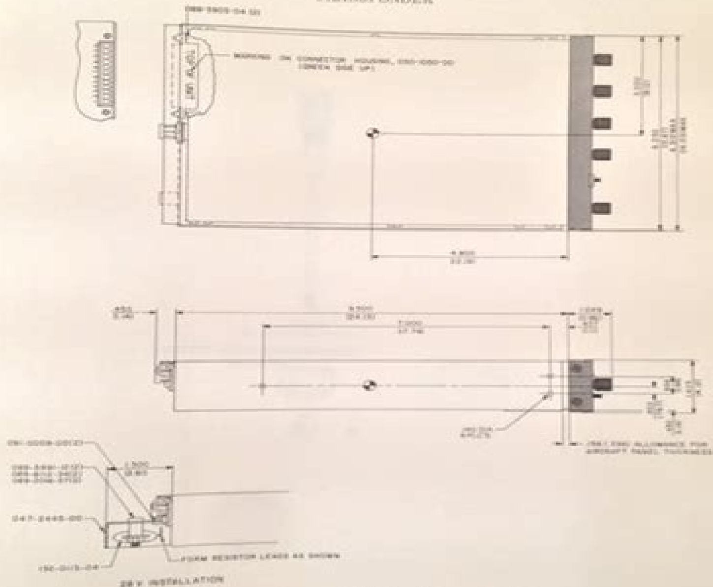
FIGURE 2-4 KT 76/78 OUTLINE AND MOUNTING DRAWING (Dwg. No. 155-5095-00 R-1)
