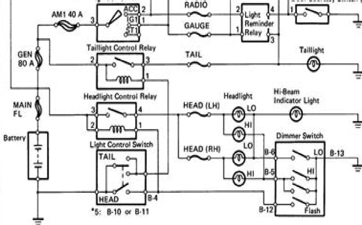
Tailight Control Relay
