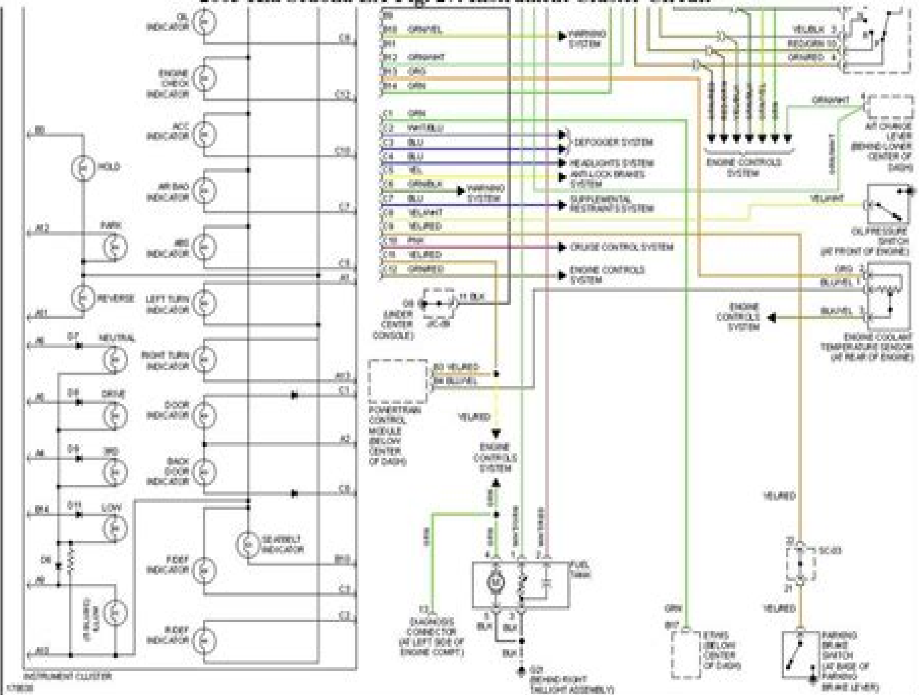
2003 Kia Sedona EX-Fig. 27: Instrument Cluster Circuit
