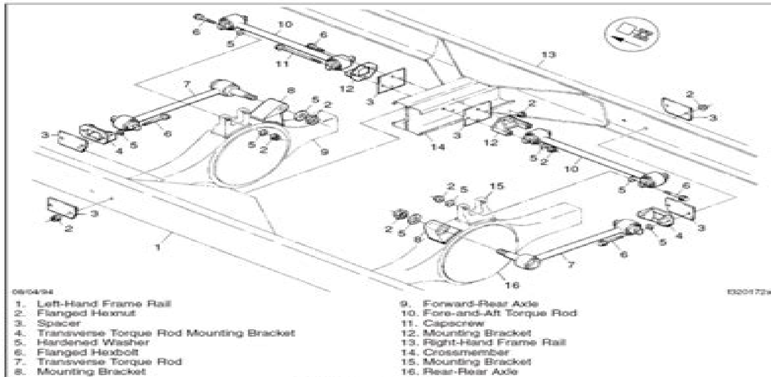
Fig. 1, Torque Rods Mounting
