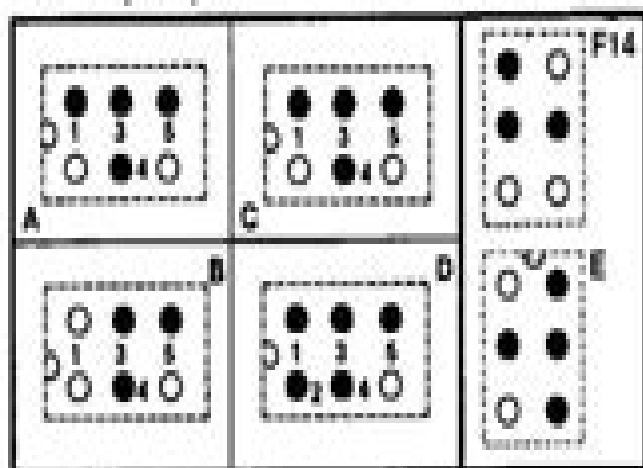
Auxiliary Relay Box
