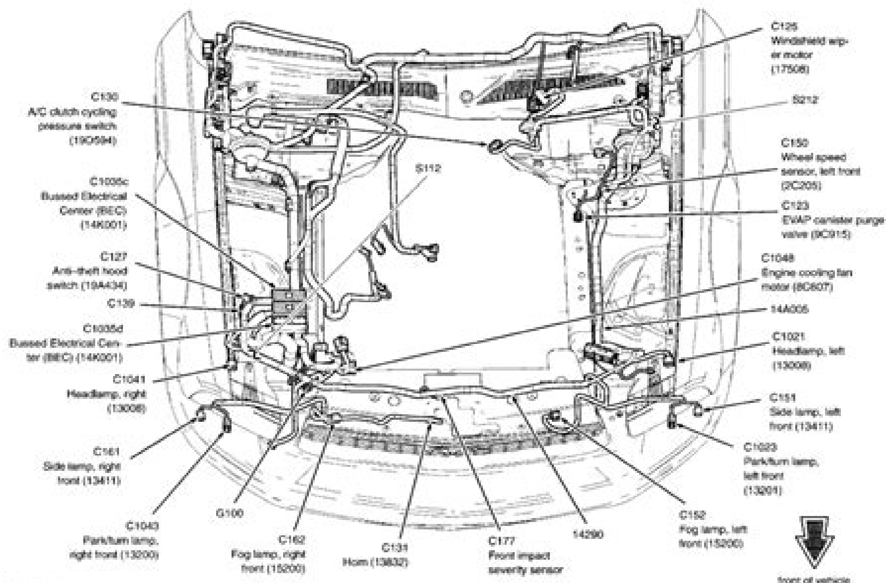
Fig 1: Engine Compartment
