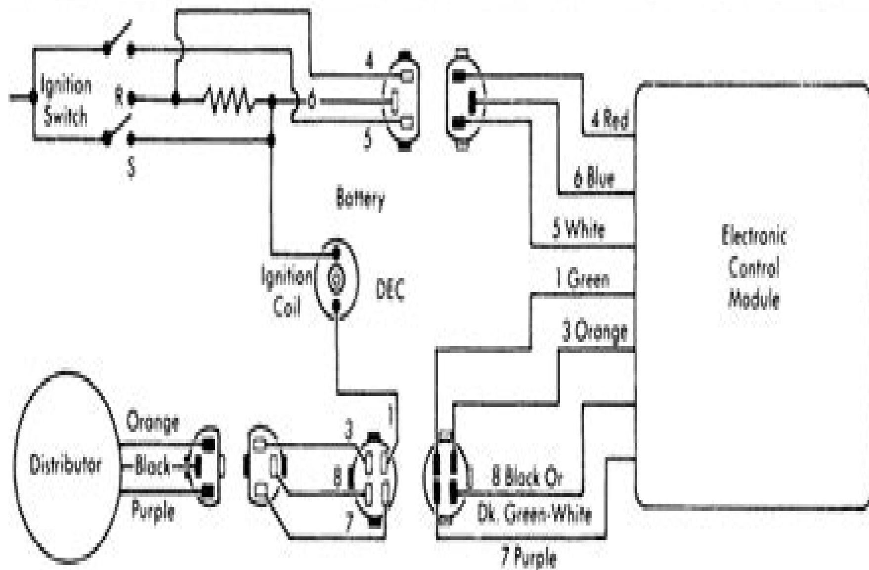
Fig. 1: 1975 Motocraft Solid State Ignition System Wiring Diagram
