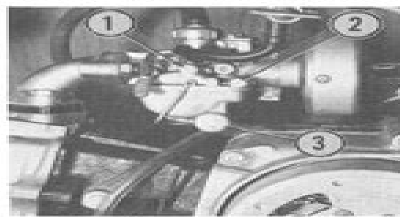
Fig. 2—Carburetor may be drained by turning drain plug (3). For adjustment of speed screw (1) and idle mixture needle (2), refer to engine section.
