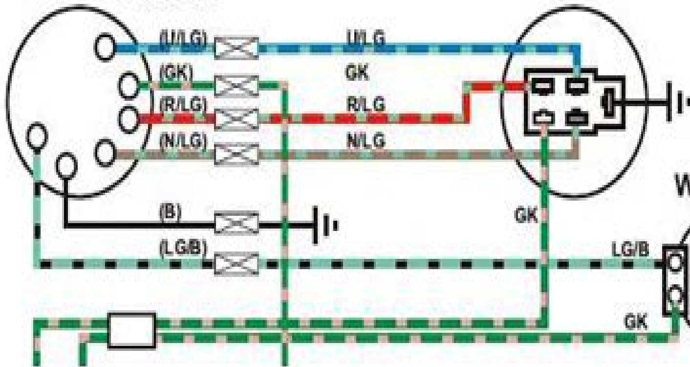
† WIPER/WASHER SWITCH
