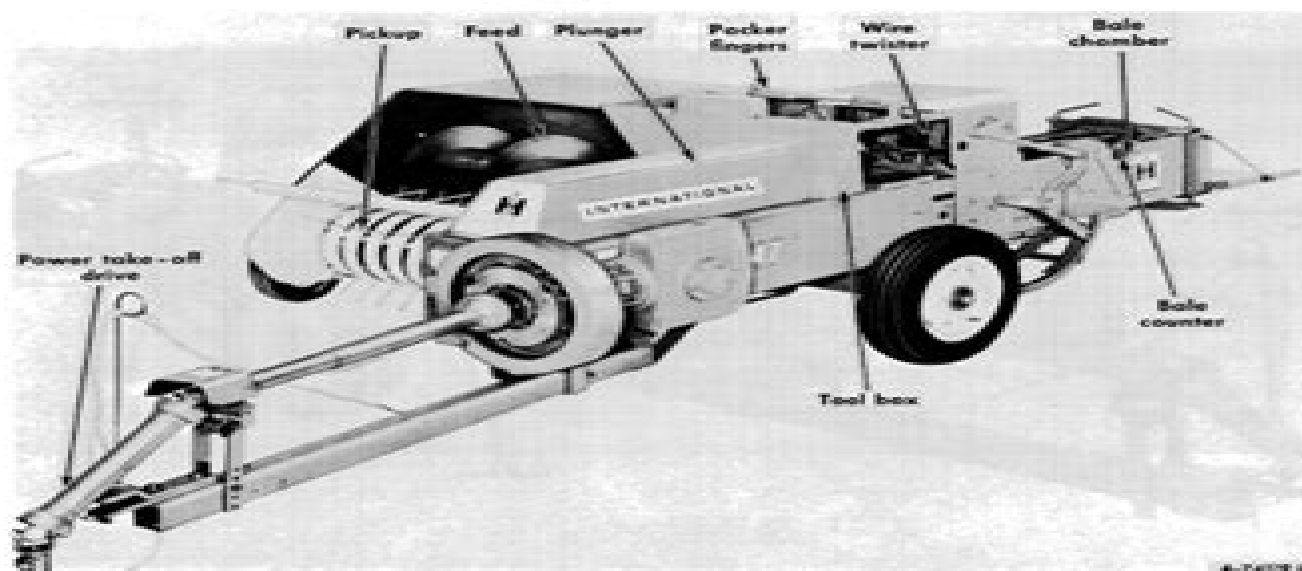
Illustr. 4 Left front view of the 47 Wire Baler.
