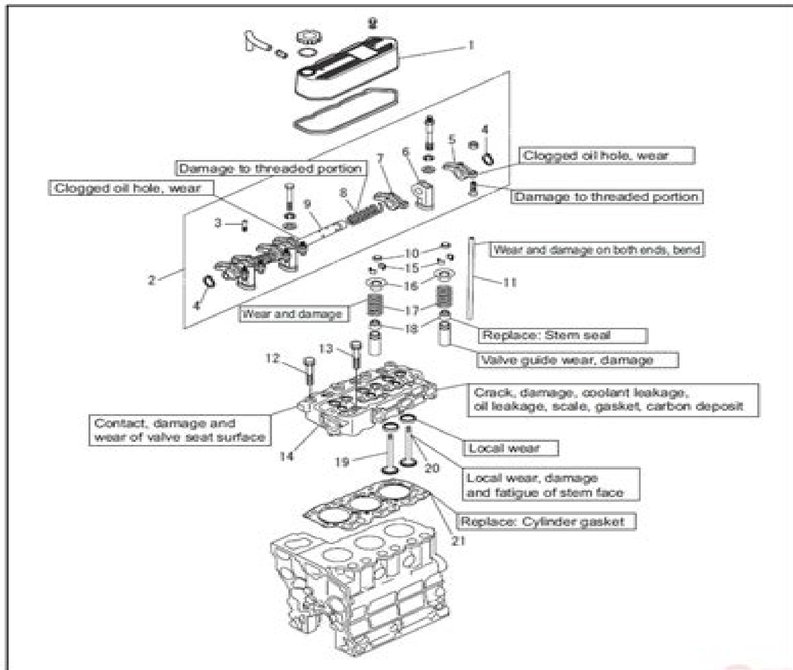
Disassembling and inspecting cylinder head and valve mechanism Disassembling sequence
