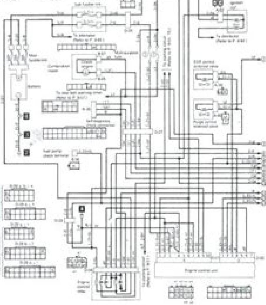
20.11a Fuel injection circuit (2.4L engine - 1 of 2)
