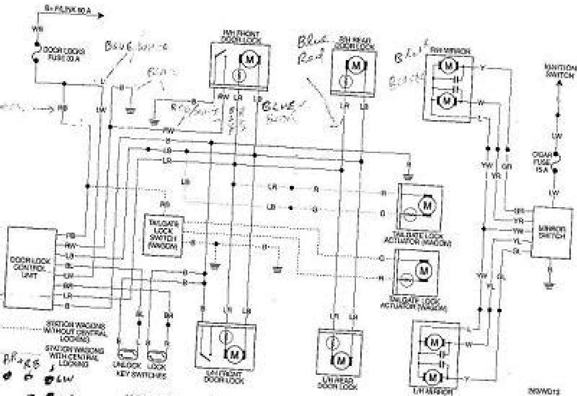
Wiring diagram for the electric mirrors and locking systems.
