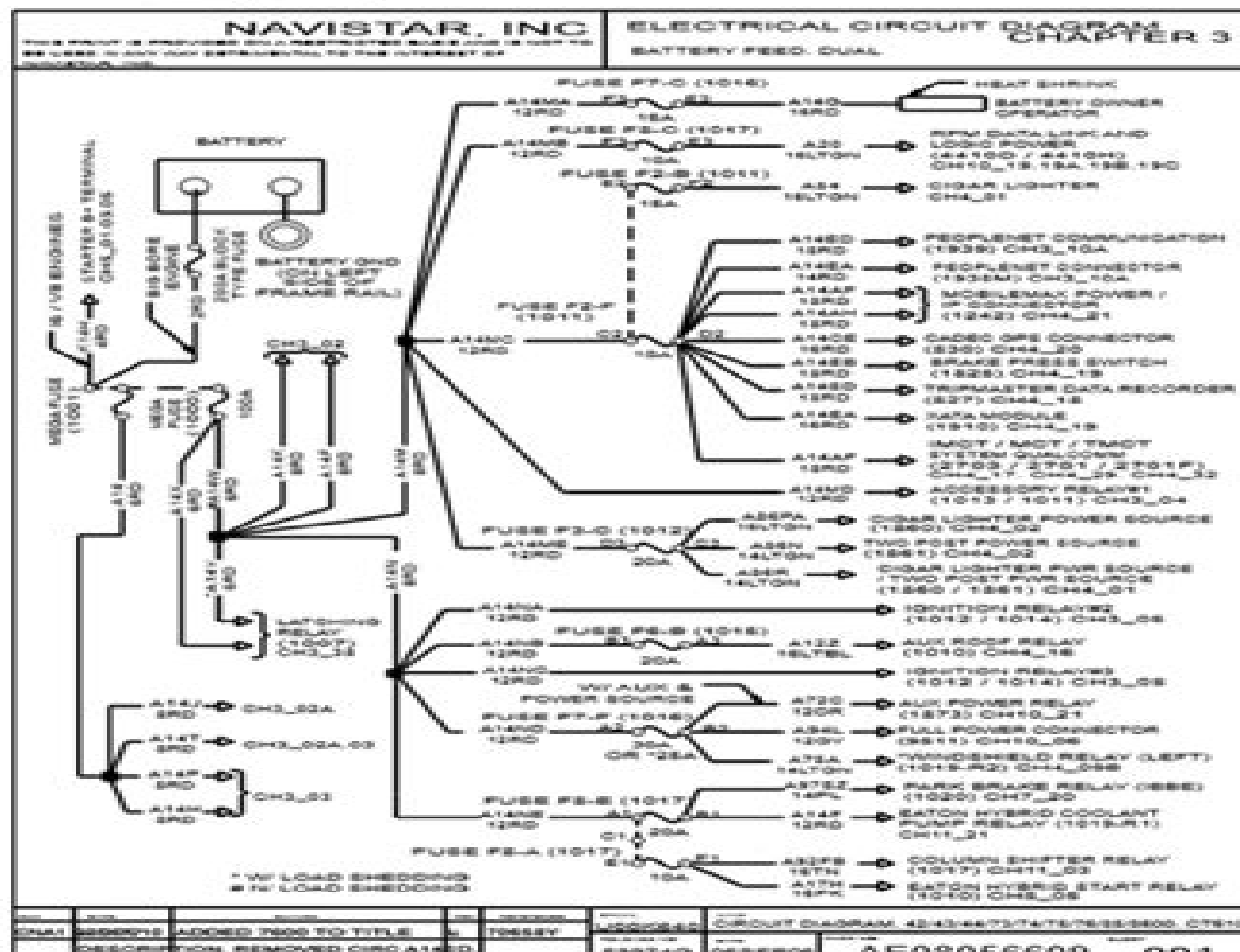
Figure 13 Battery Feed, Dual
