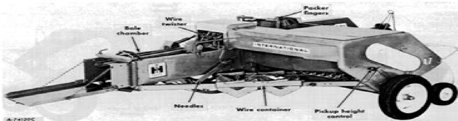
Illustr. 4A Right rear view of the 47 Wire Baler shows with four-cell wire container. Baler can be obtained with two-cell wire container.
