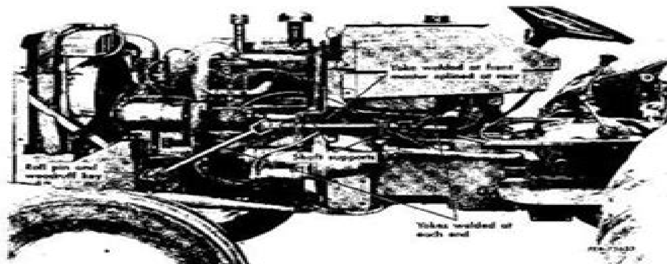
Illust. 6. Steering shaft and supports, 424 shown, 404 similar.
