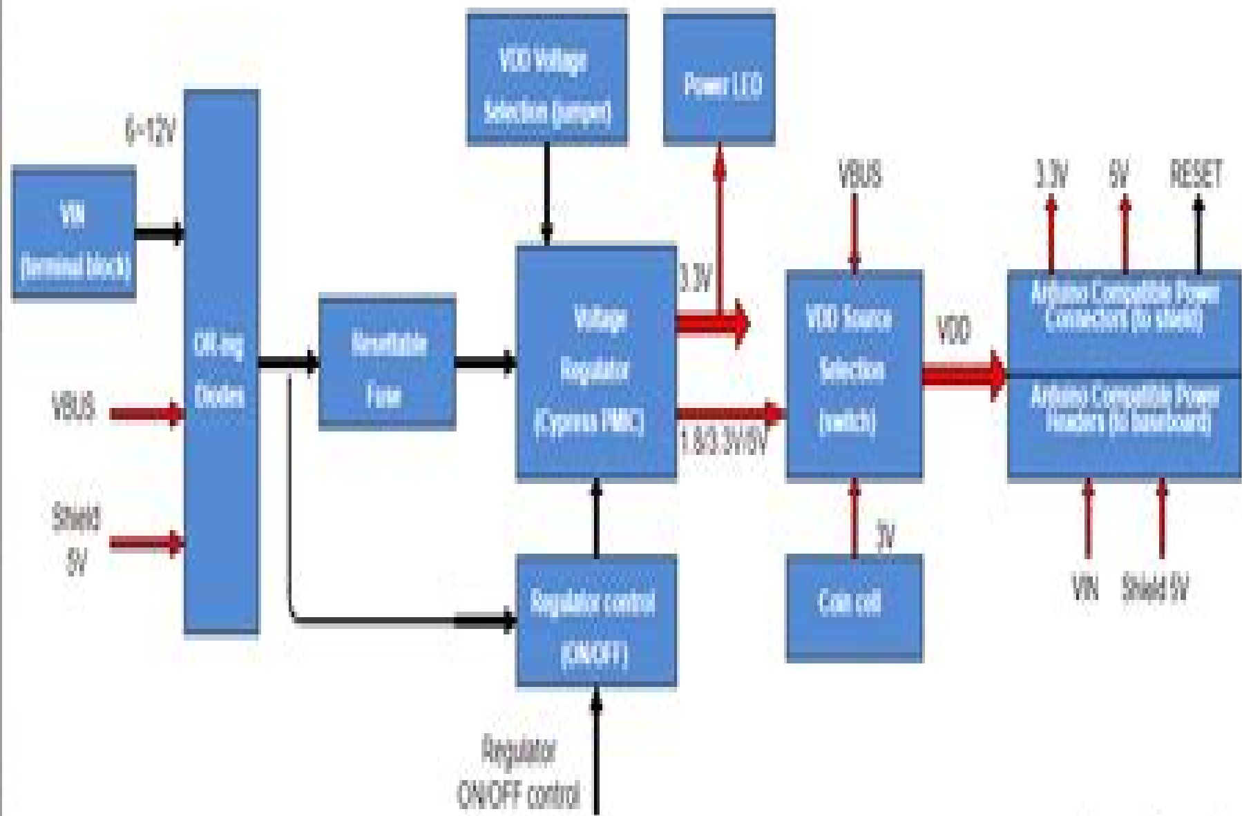
Power Supply
