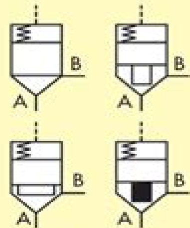
Logic Operators
