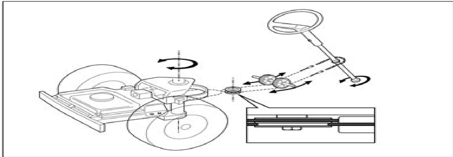
Outline diagram of the articulated steering function.
