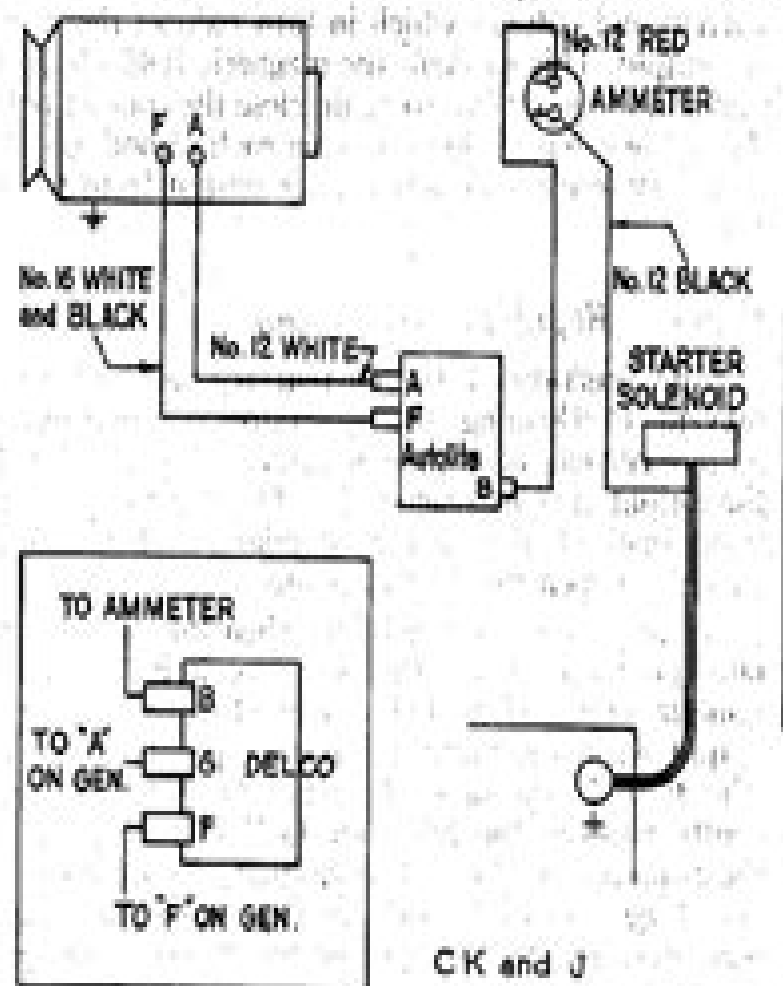
GENERATOR CIRCUIT
