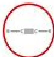
ALKYNE
