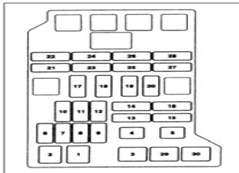
Fig 2: Identifying Engine Compartment Fuses
