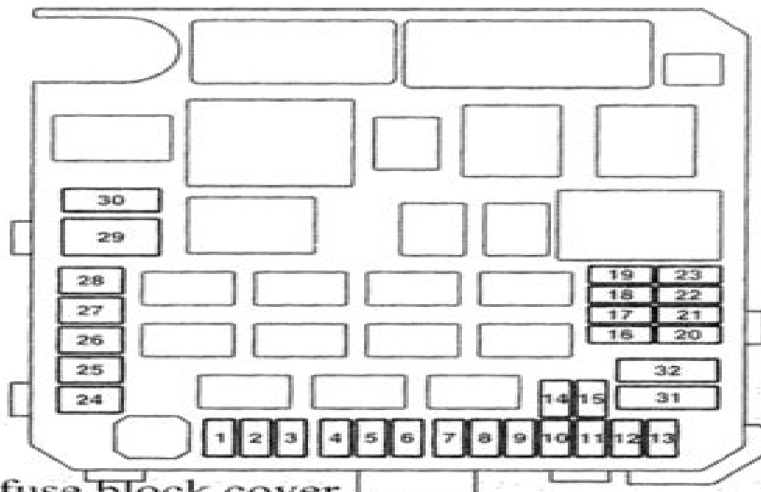
Fig 5: Identifying Location Of Engine Compartment Fuses Engine compartment fuse location
