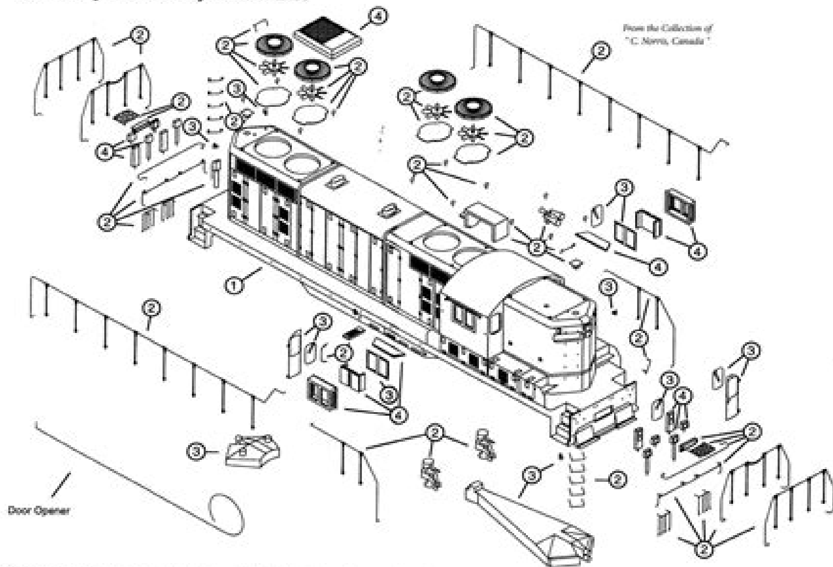
FIG. 1A Exploded Parts Drawing GP7 Body Shell with Dynamic Brakes
