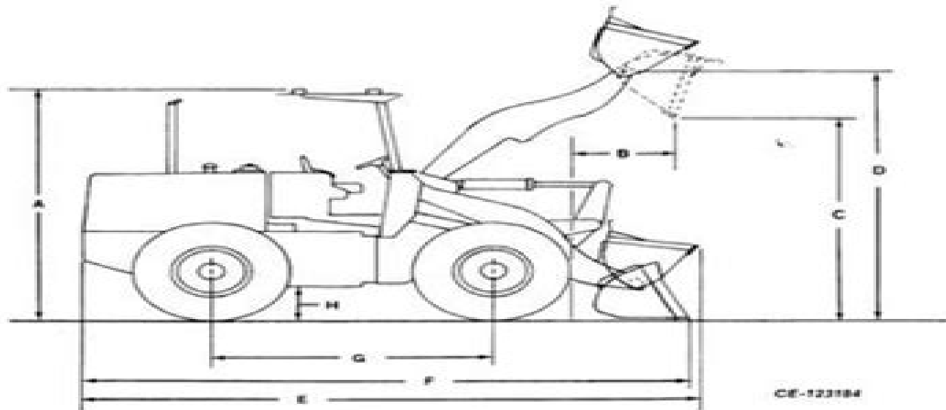
FIG. 1 — General Dimensions
