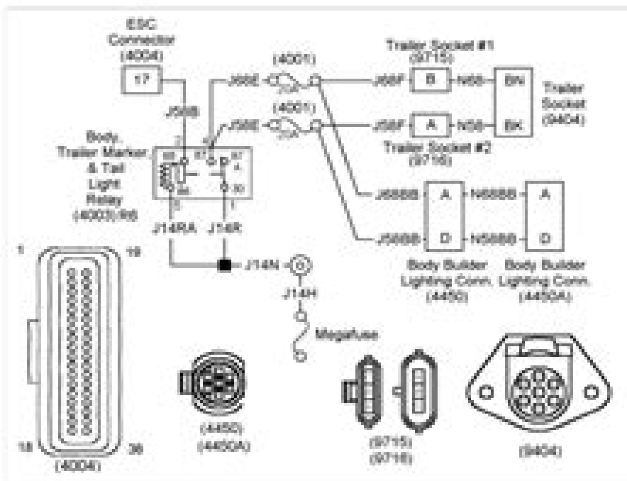
Figure 3-48 Body, Trailer Marker & Tail Light Relay Circuits—Always Refer To Circuit Diagram Book For Latest Circuit Information
