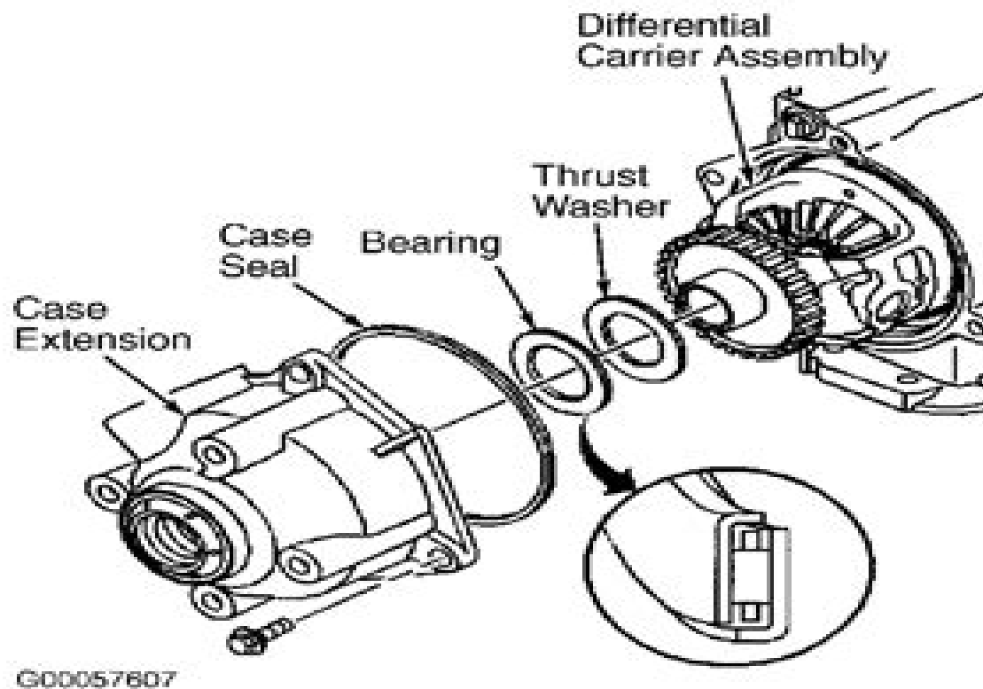
Fig. 19: Removing & Installing Case Extension Courtesy of GENERAL MOTORS CORP.
