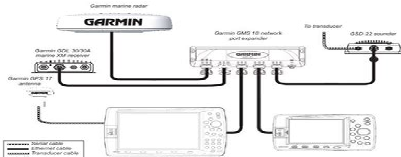
The Garmin Marine Network with Multiple Devices and a GSD 22
