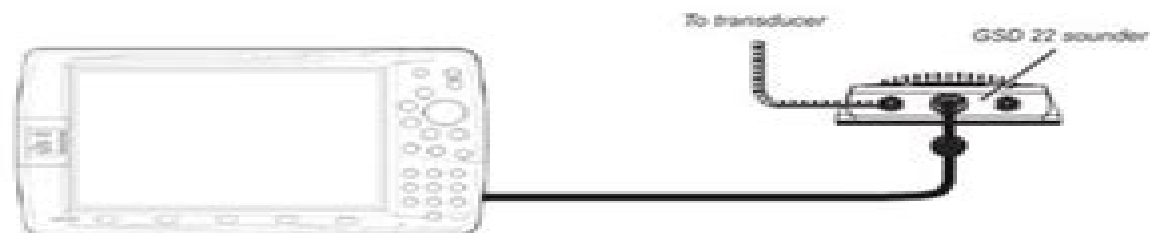
The Garmin Marine Network with a Single Chartplotter and a GSD 22
