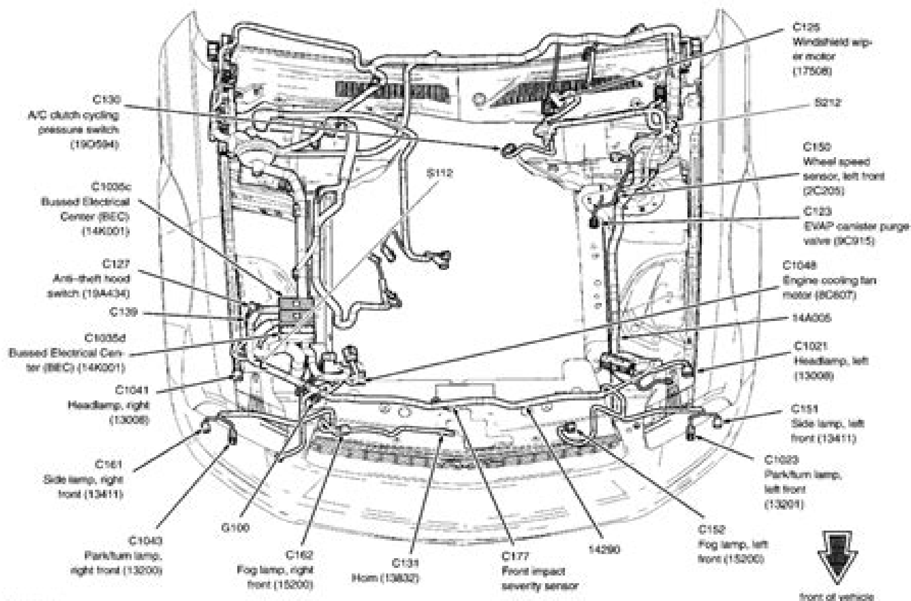
Fig 1: Engine Compartment
