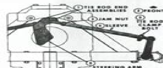
Fig. 3—View showing position of all purpose type center steering arm for checking toe-in. Note that center arm (8) and tie rod inner ends are different than those used on row crop front end. View is from top.
