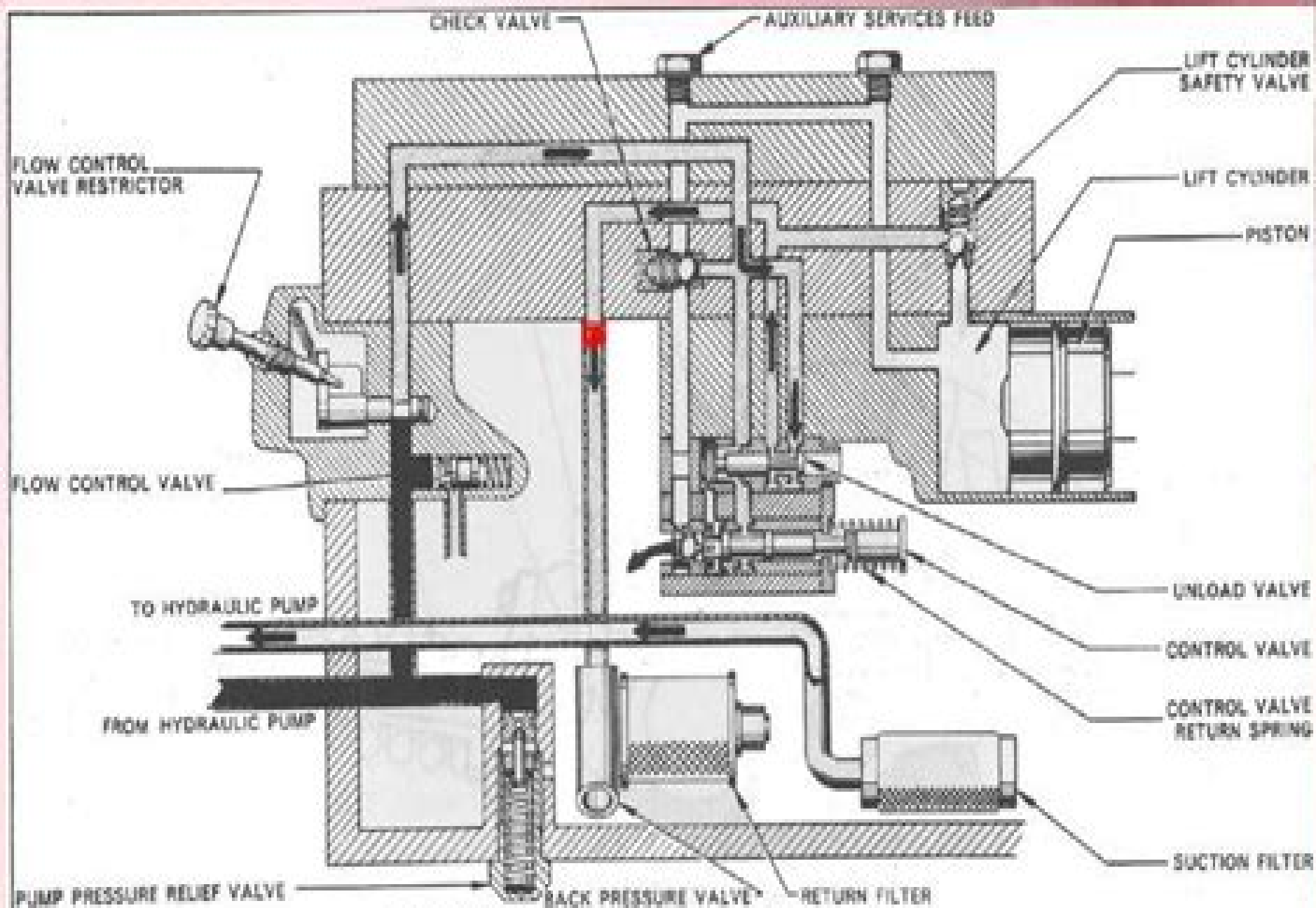
FIGURE 9. OIL FLOW IN NEUTRAL
