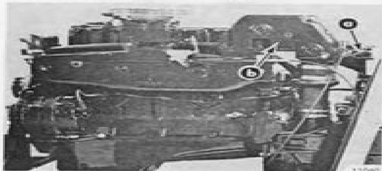
a - Shift Plate On Inner Transom Plate b - Straight-Back Exhaust Elbow
