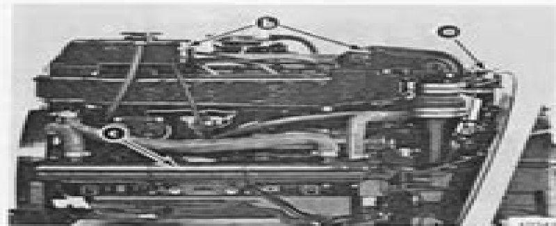
a - Shift Plate Mounted On Inner Transom Plate b - Separate Coolant Reservoir and Exhaust Elbow c - 3" (76mm) Heat Exchanger
