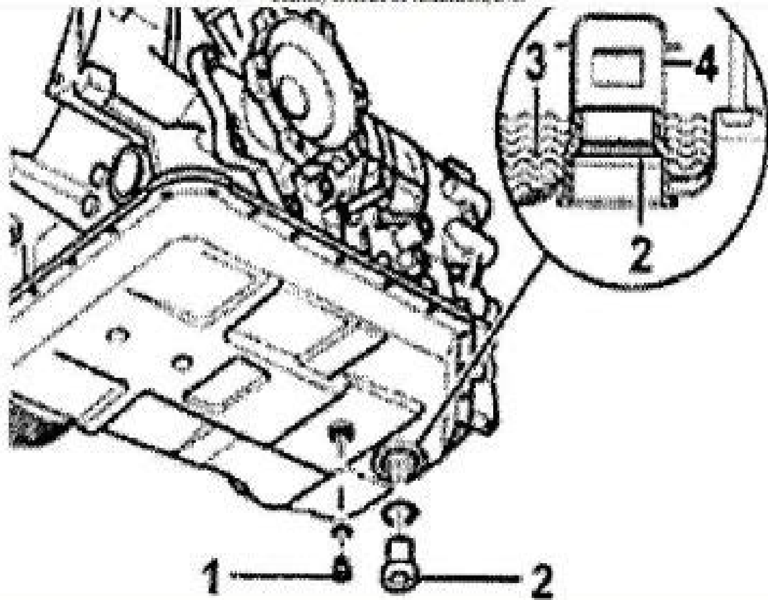
Fig. 4: Locating Transaxle Drain Courtesy of AUDI OF AMERICA, INC.
